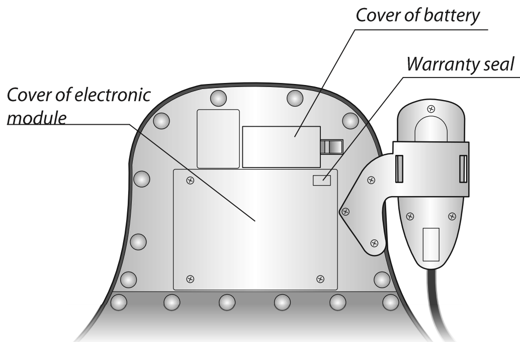
Fig. 2. Module of electrostimulation (bottom view of the part, which contains electronic unit)
