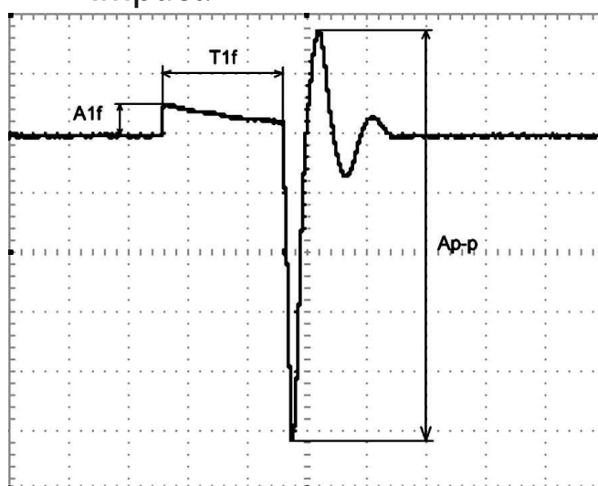
Pulse form under connected load Z
